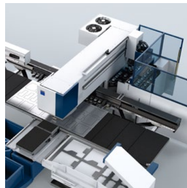
Automatic tool change with the ToolMaster Linear.
